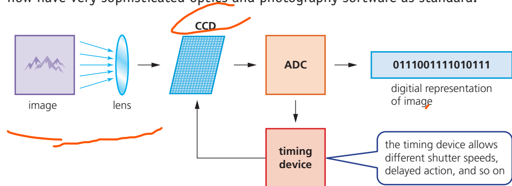
▲ Figure 3.22 Diagram of how a digital camera works
